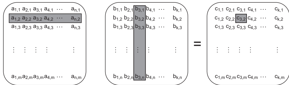
Figure 8.3 Matrix multiplication
